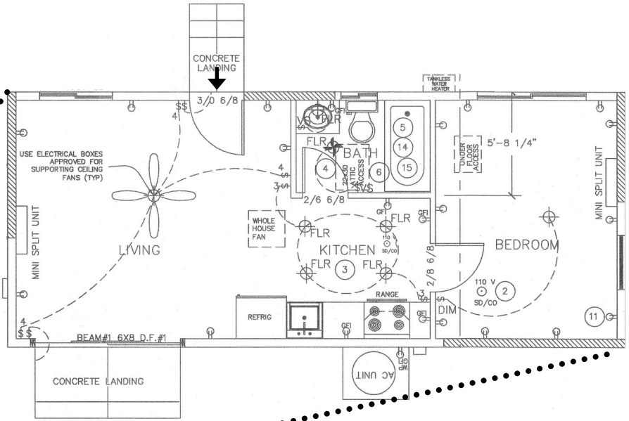
Accessory Dwelling Unit Floor Plan
