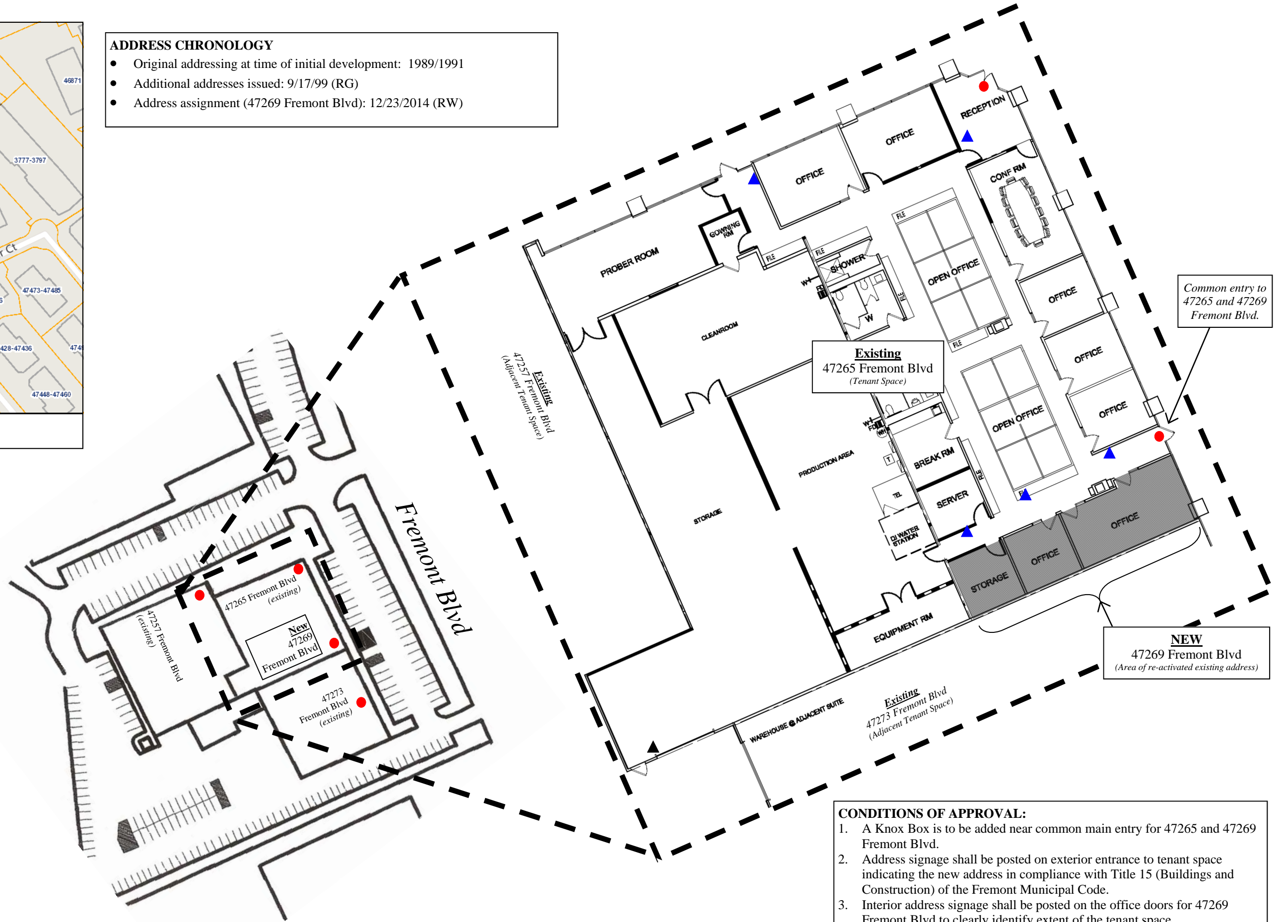
LOCATIONAL MAP
