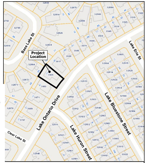
LOCATIONAL MAP
