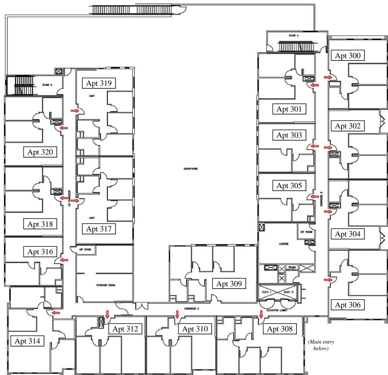
Third Floor
