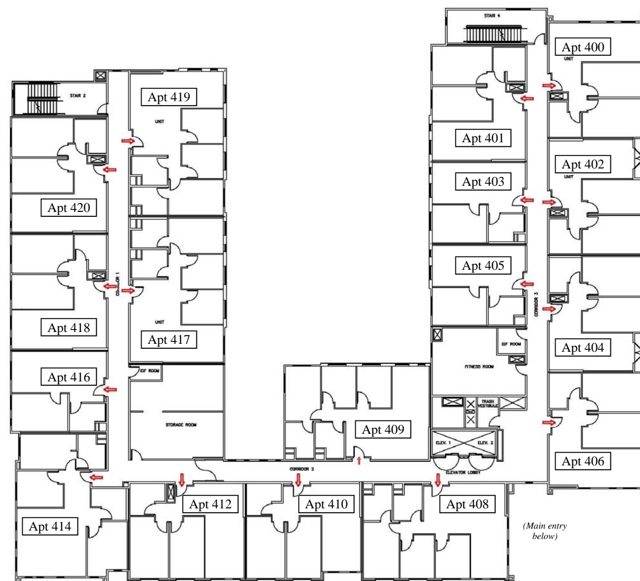
Fourth Floor
